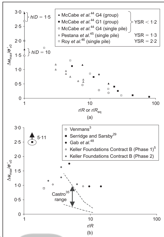
Figure 6. Maximum excess pore pressures around: (a) driven piles in clay, 33 (b) stone columns
