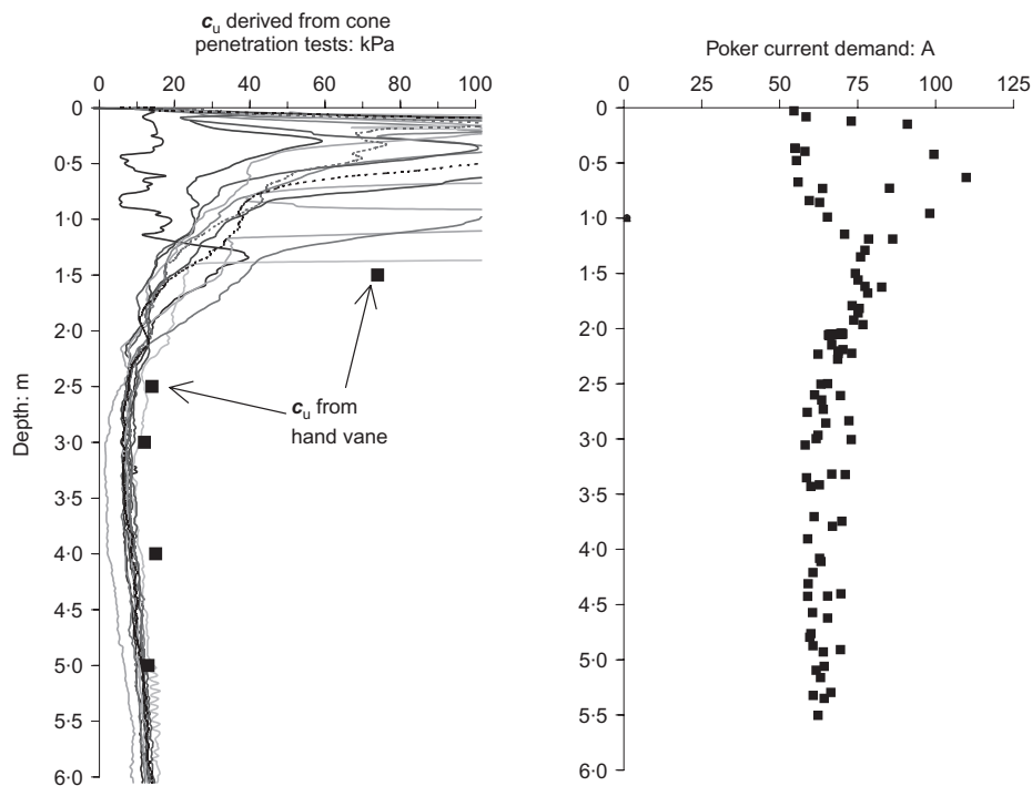
Figure 3. Relationship between undrained shear strength and current demand of poker 5
