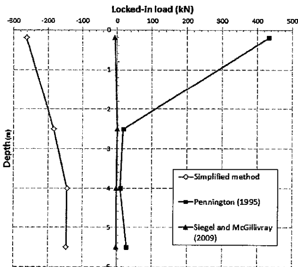
Figure 6 – Comparison of derived residual loads using interpretation methods
