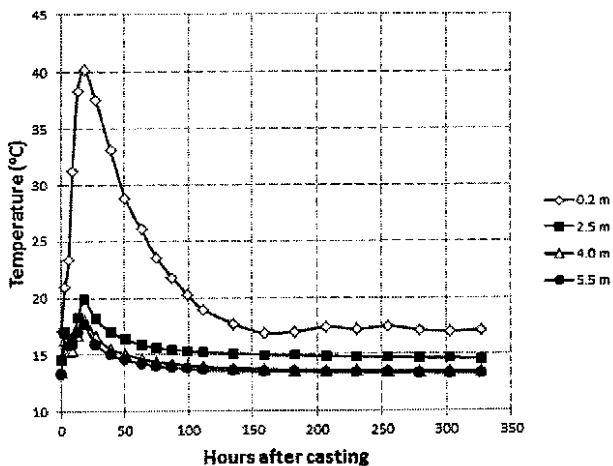
Figure 3 – Variation in temperature after casting
