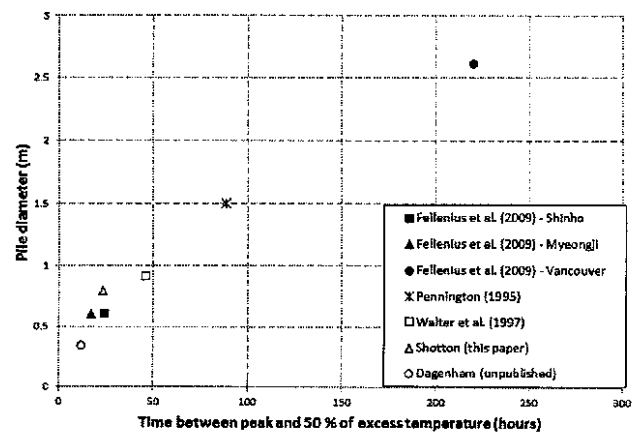
Figure 2 – Variation in time between peak and 50 % of excess temperature with pile diameter
