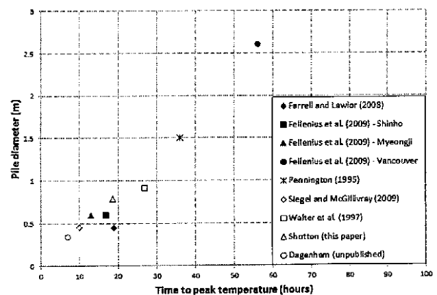
Figure 1 – Variation in time to peak temperature with pile diameter
