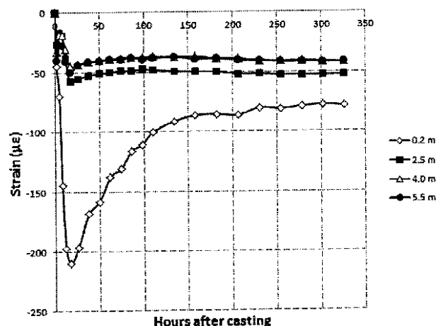
Figure 5 – Variation in temperature-corrected strain after casting
