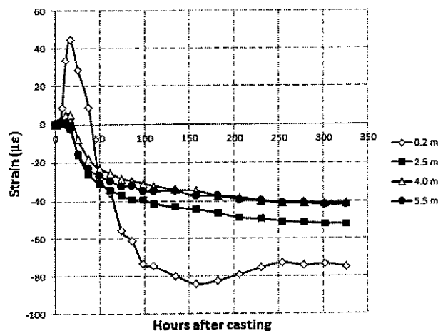
Figure 4 – Variation in total (uncorrected) strain after casting
