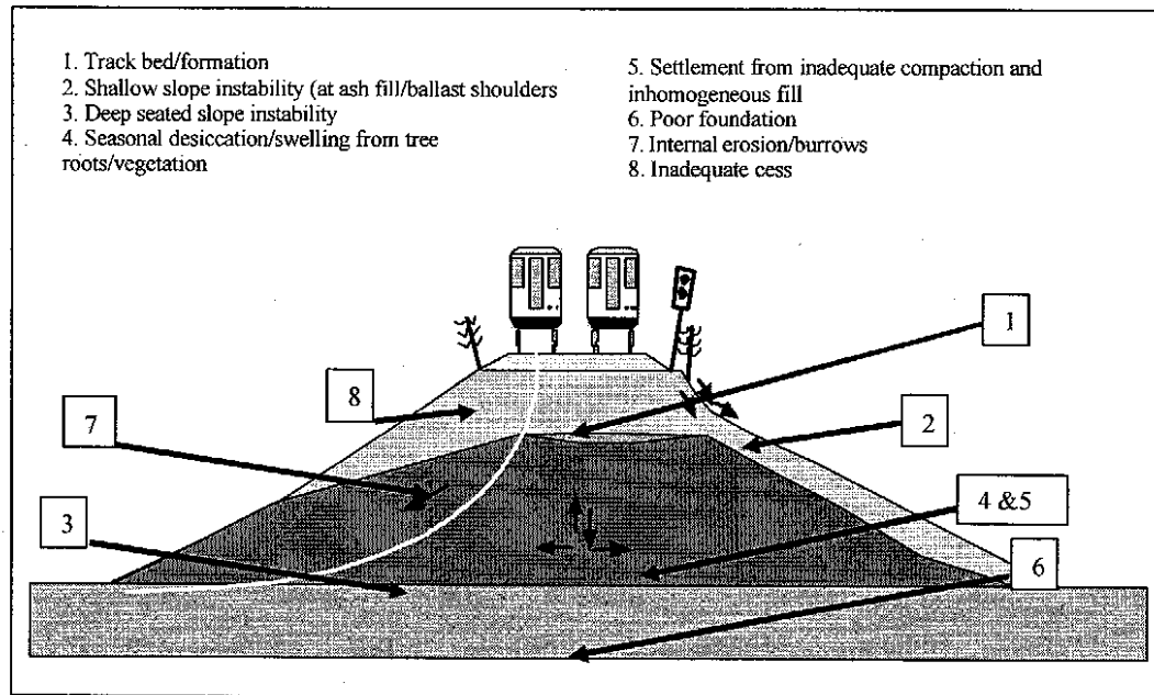
Figure 6 Typical embankment deformation mechanisms.
