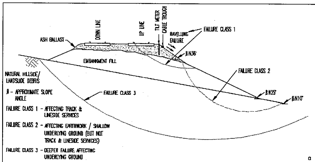
Figure 7 Failure types affecting Ilkley Embankment
